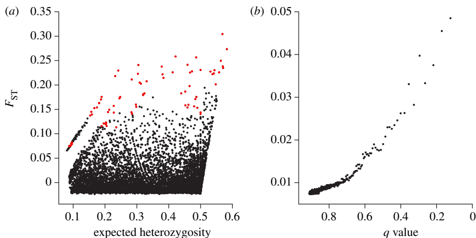
Figure 4. F_{ST} outlier test results of (a) FDIST2 and (b) BAYESCAN, showing loci detected as putatively under directional selection based on a FDR of 0.1 (red circles; only FDIST2 found loci putatively under selection).
