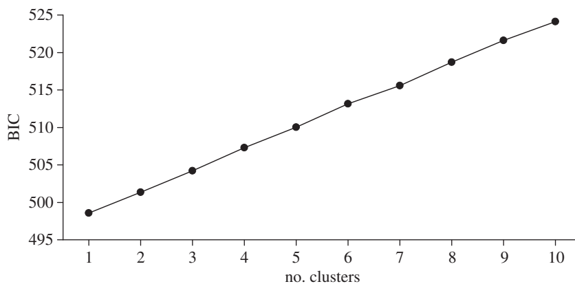
Figure 3. Inference of the number of genetic clusters using Bayesian information criterion (BIC) in the R package ADEGENET for DAPC analysis. The optimal clustering solution corresponds to the lowest BIC, which in this case is one cluster.
