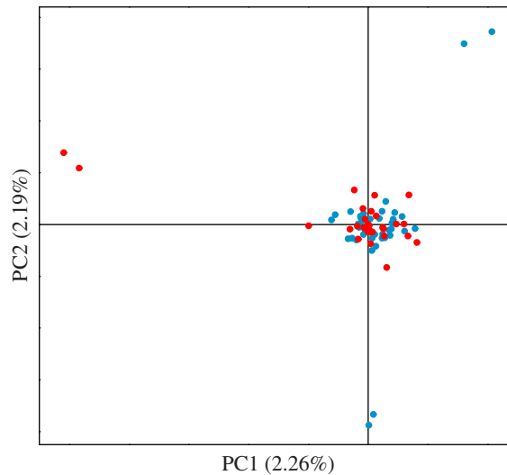
Figure 2. PCA from 8294 SNPs of pygmy blue whales from the Australian feeding aggregations (red, Bonney Upwelling; blue, Perth Canyon).
